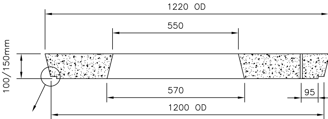
SECTION THROUGH LID
