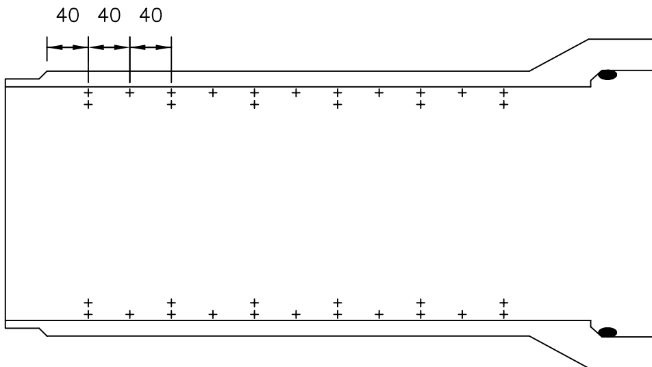
225 \phi CONCRETE PERFORATED PIPE
